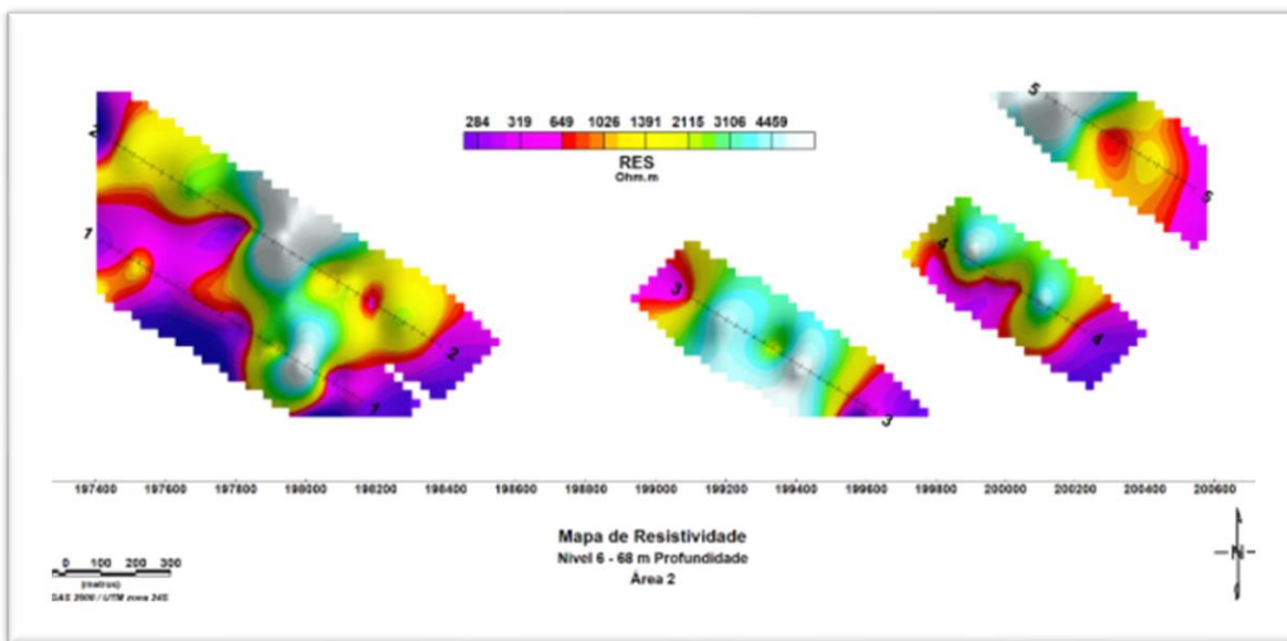
Figure 9-12 Depth Map of Real Resistivity (N6 = 68 m)
