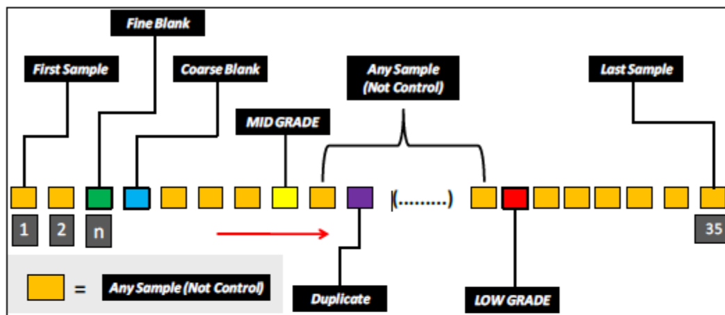
Figure 11-1 Logical Sequence Matrix
