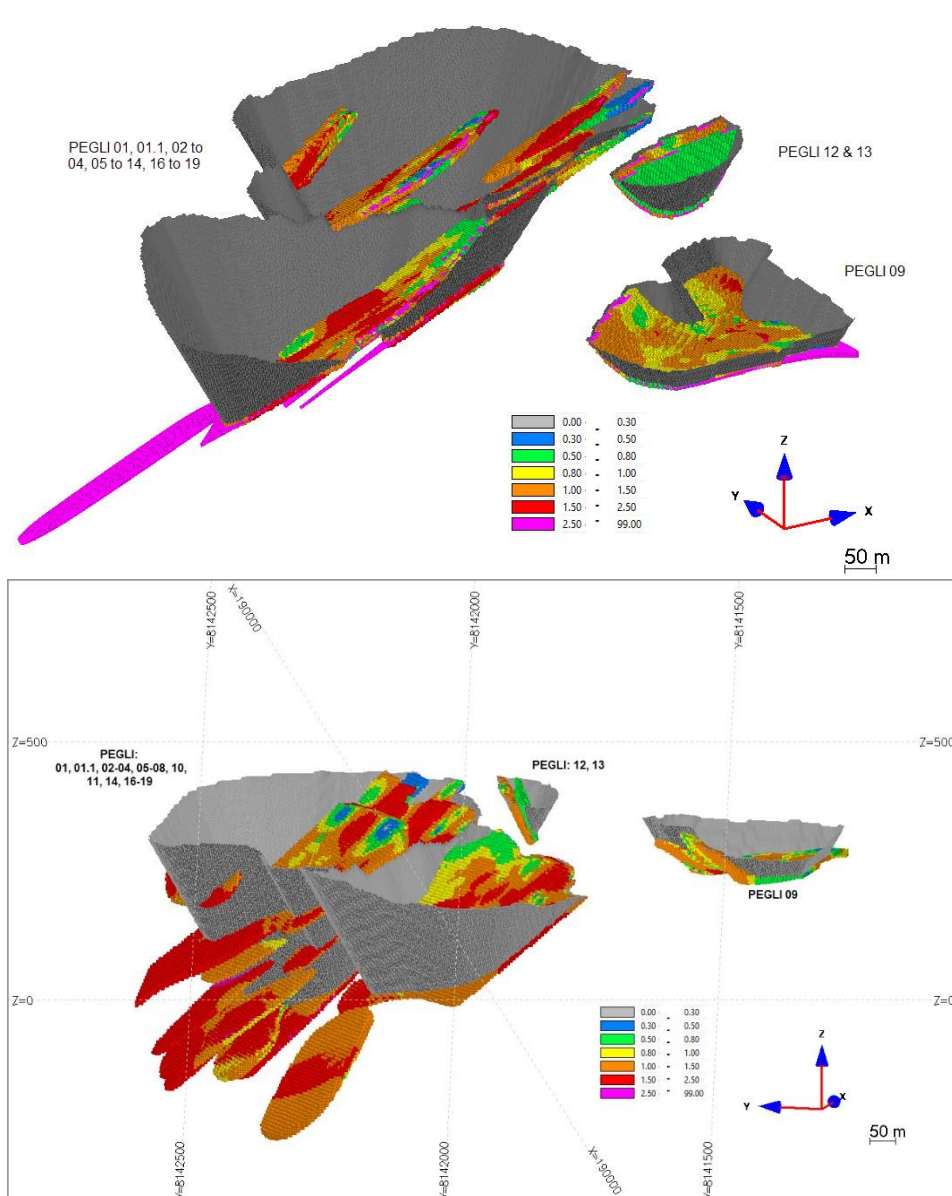
Figure 14-10 Isometric View Looking Northwest: Bandeira Deposit Mineral Resource Block Grades and Whittle Pit
