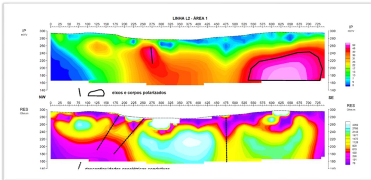
Figure 9-7 Depth Model of the Chargeability (Top Panel) and the Actual Resistivity (Bottom Panel) of Line 2 of Area 1
