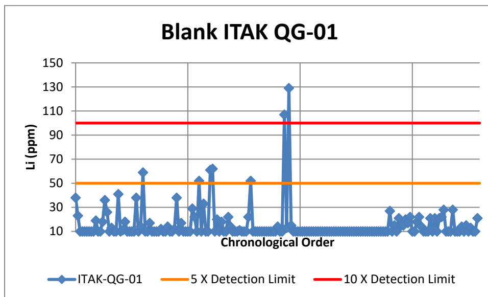
Figure 11-6 Coarse Blank Sample Chart for Li (ppm)
